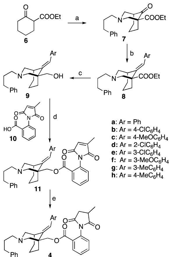
Scheme 1. (a) 3-phenylpropylamine, paraformaldehyde, AcOH, EtOH, H 2 O (49%); (b) ArCH 2 PO(OEt) 2 , n BuLi, THF, room temp., ovn or, for 8f , reflux ovn, 8a (84%), 8b (99%), 8c (31%), 8d (76%), 8e (68%), 8f (15%), 8g (10%), 8h (42%); (c) LiAlH 4 , THF, 9a (99%), 9b (98%), 9c (74%), 9d (61%), 9e (95%), 9f (91%), 9g (95%), 9h (79%); (d) 10 , DCC, DMAP, CH 2 Cl 2 , 11a (76%), 11b (57%), 11c (58%), 11d (53%), 11e (60%), 11f (82%), 11g (63%), 11h (63%); (e) H 2 , Pd/C, EtOAc, 4a (88%), 4b (73%), 4c (68%), 4d (47%), 4e (55%), 4f (57%), 4g (71%), 4h (79%).
